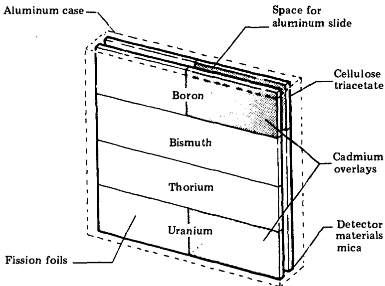
Figure 3-6 Neutron Detector
