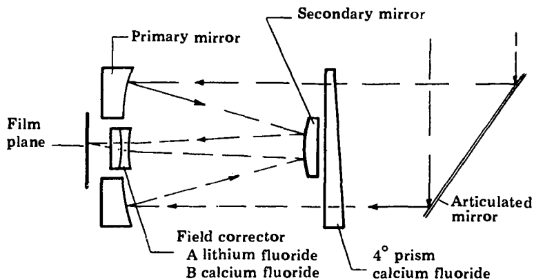
Figure 4-1 Optical Plan
